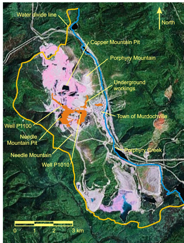
Figure 6.6. Satellite image showing the surface area covered by the underground mine workings of the Gaspé Mines (Raymond, 2010). Source for the background image: earth.google.com.
